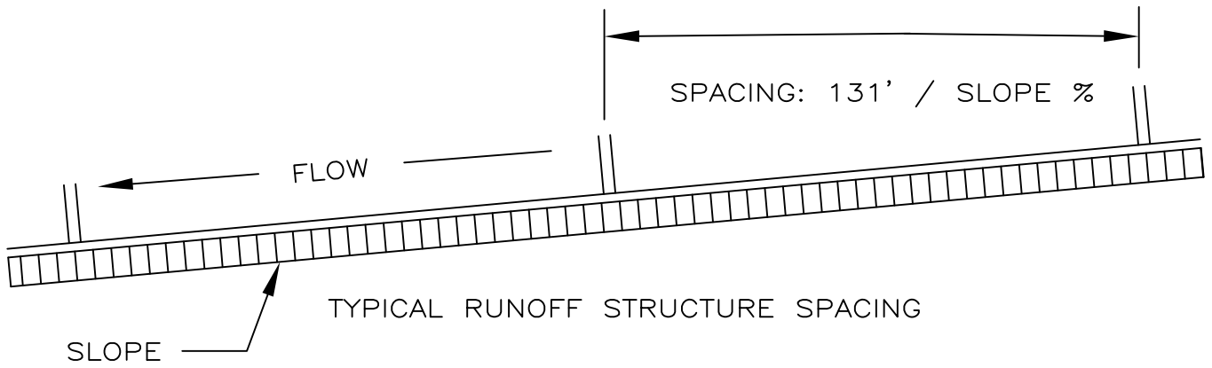
CROSS-SECTION
