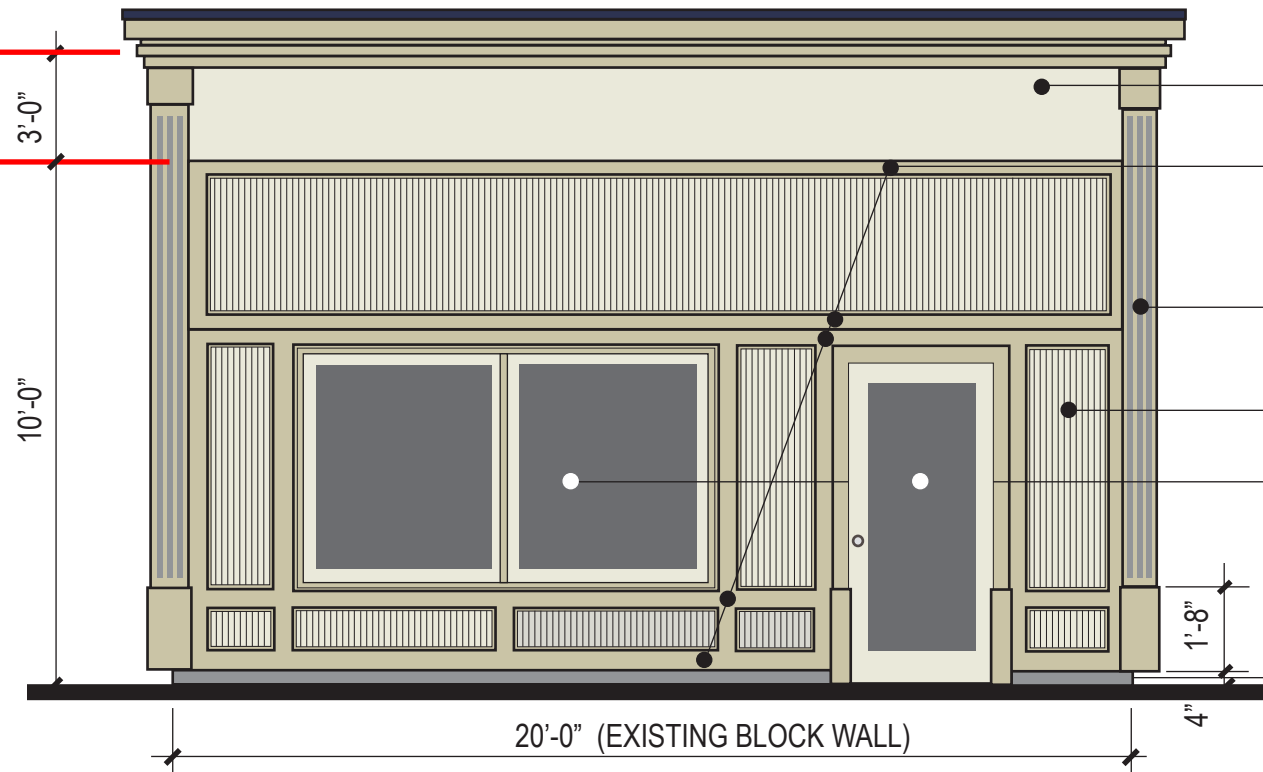
FRONT FACADE
